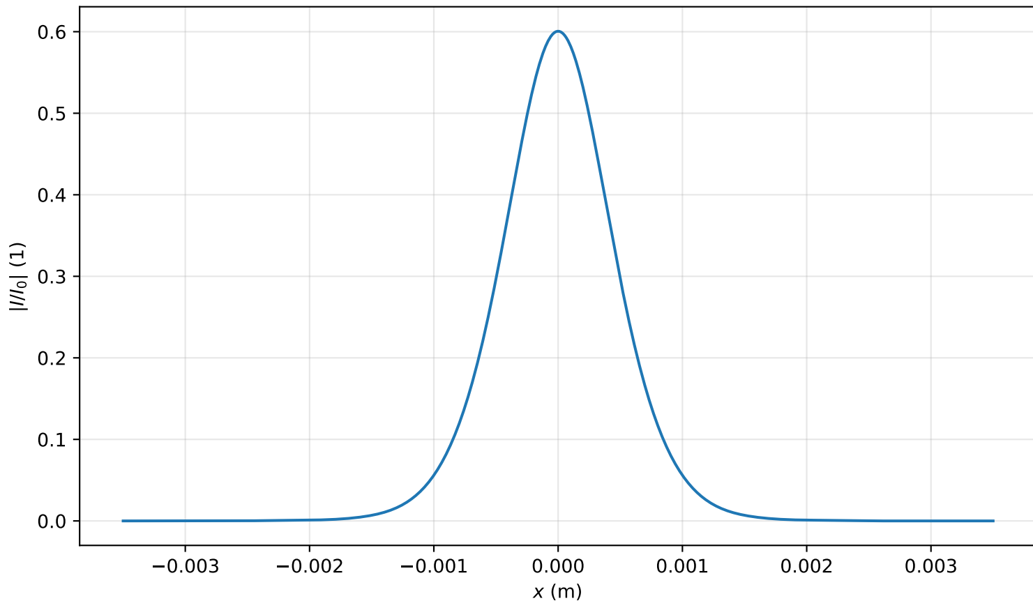
Intensity profile I(x, y = 0, z = 3.344m)/I_0 , P_{in}=0.6P_{cr} , artificial time
